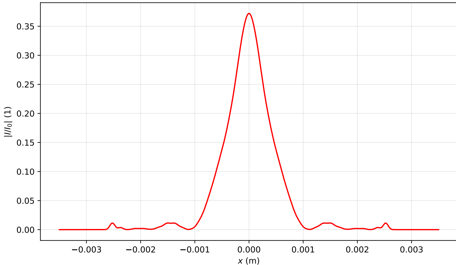
Intensity profile I(x, y = 0, z = 1.115)/I_0 , P_{in}=3.0P_{cr} , artificial time
